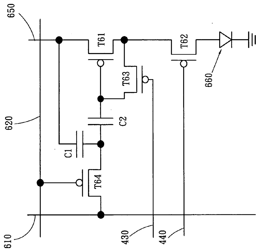
Fig. 6 PRIOR ART
